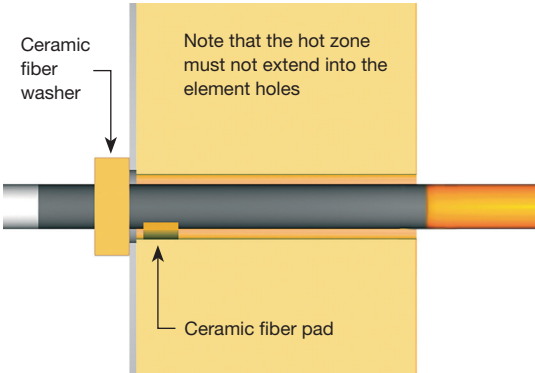
Fig. 5 Installation without sleeves.
