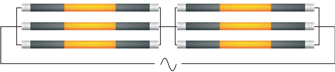
Alternative method of series/parallel connection, not recommended
