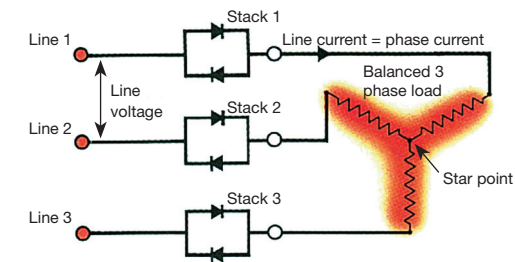
3-phase, 3-wire, star-connection (phase-angle firing) Stack voltage rating = line voltage = phase voltage \times \sqrt{3} Stack current rating = line current = phase current Note: phase resistances and loads must be balanced
