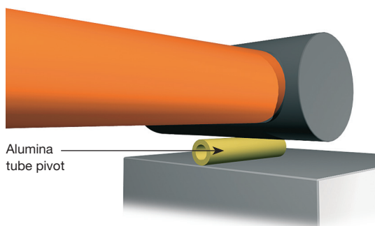
Fig. 7 Typical horizontal installation methods.
