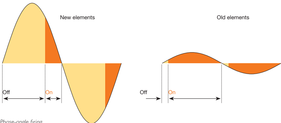
Fig. 13 Phase-angle firing.
