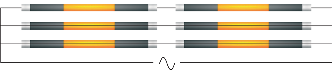
Preferred method of series/parallel connection
