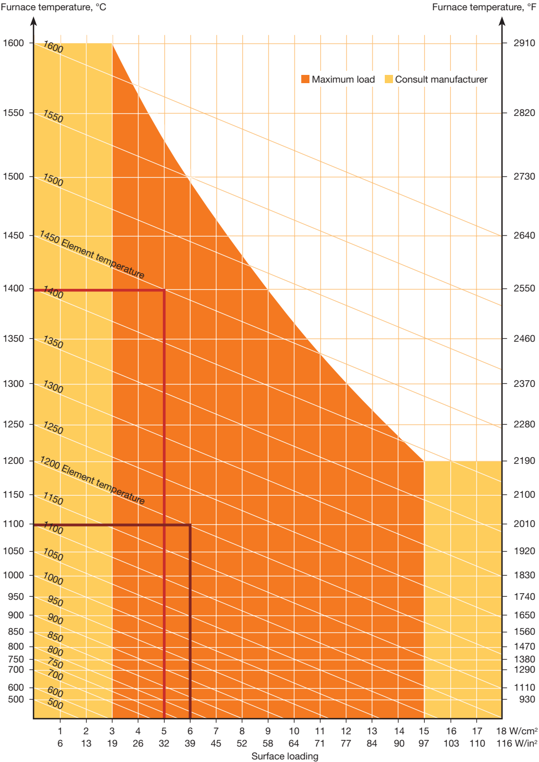
Fig. 10 Surface loading chart.
