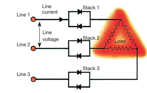
3-phase, closed delta connection Stack voltage rating = line voltage Stack current rating = line current = phase current \times \sqrt{3}
