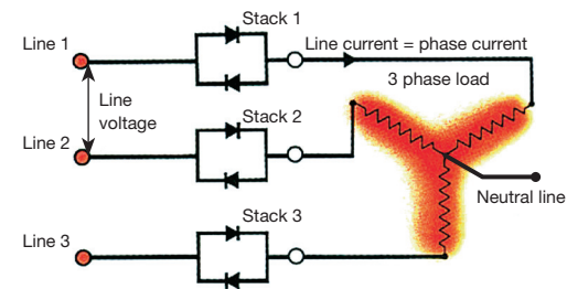
3-phase, 4-wire, star-connection (phase-angle firing) Stack voltage rating = phase voltage = \frac{\text{line voltage}}{\sqrt{3}} Stack current rating = line current = phase current Neutral cable rating = line current \times 2 for safety
