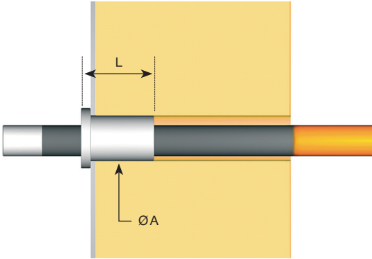
Fig. 4 Standard sleeve patterns and installation.
